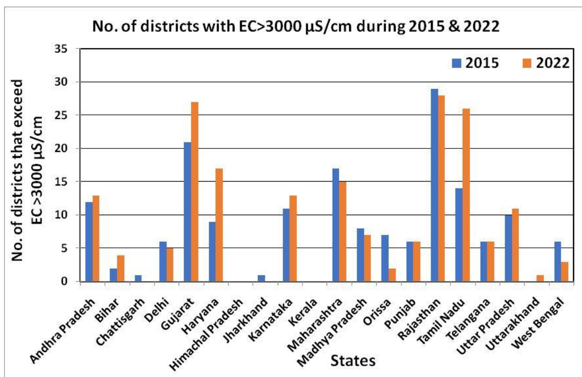
Fig. 7.1.4 Comparison on No of districts exceed EC >3000 \mu\text{S}/\text{cm} during 2015 and 2022.
